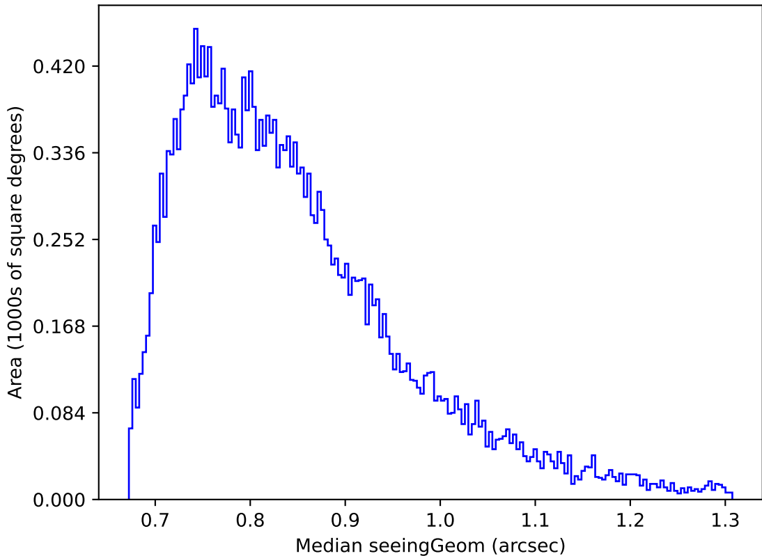
too_elab_r16_d3_ugrizy_v3.4_10yrs Yr 1 i band: Median seeingGeom
