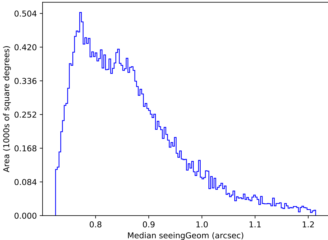
too_elab_r16_d3_ugrizy_v3.4_10yrs Yr 1 all bands: Median seeingGeom
