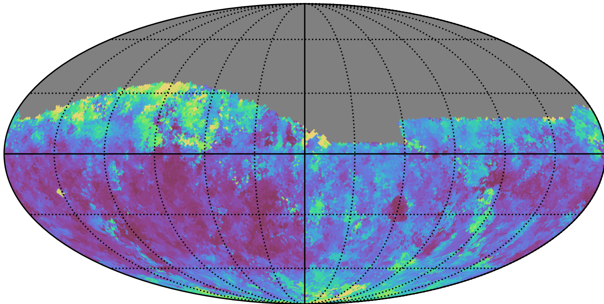
too_elab_r16_d3_ugrizy_v3.4_10yrs Yr 1 z band: Median seeingEff
