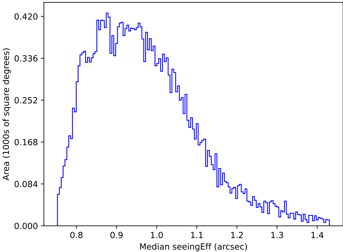
too_elab_r16_d3_ugrizy_v3.4_10yrs Yr 1 z band: Median seeingEff
