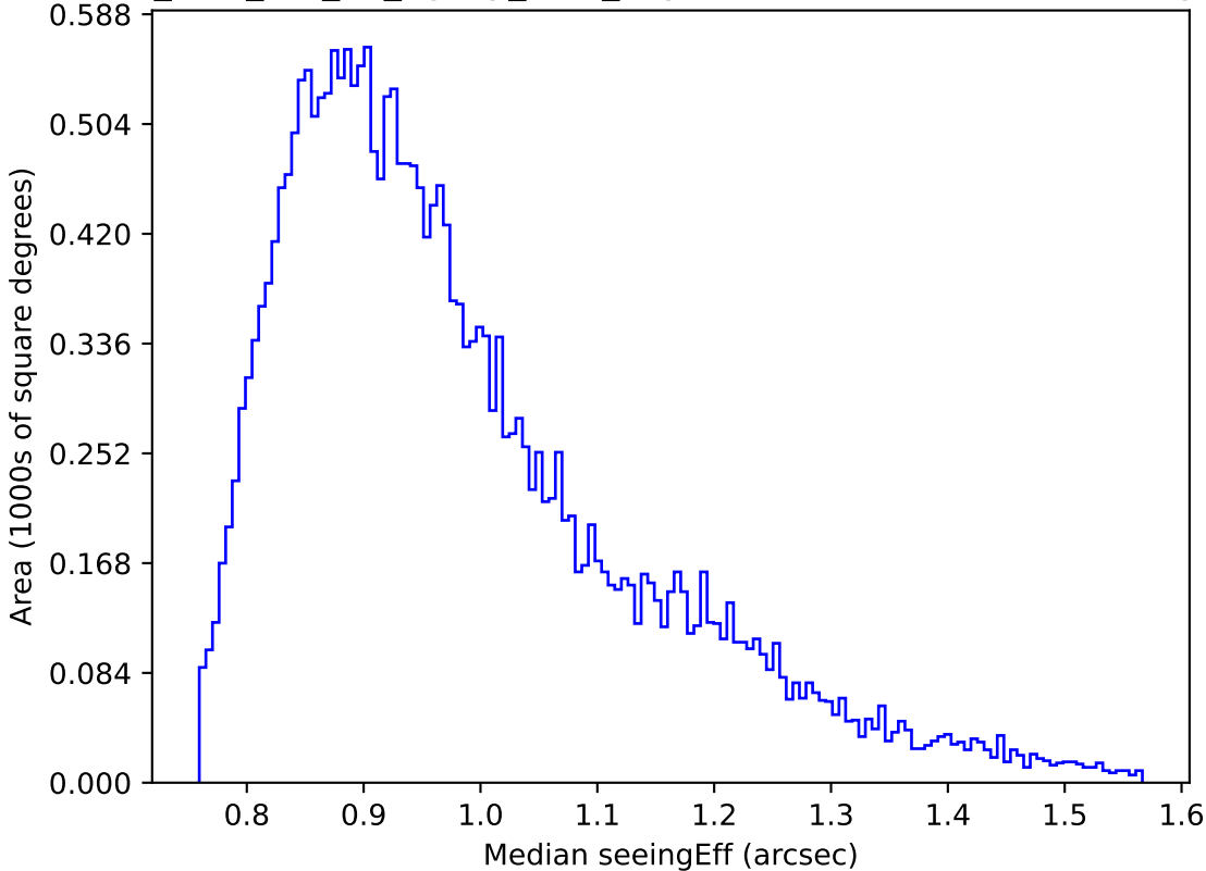
too_elab_r16_d3_ugrizy_v3.4_10yrs Yr 1 r band: Median seeingEff
