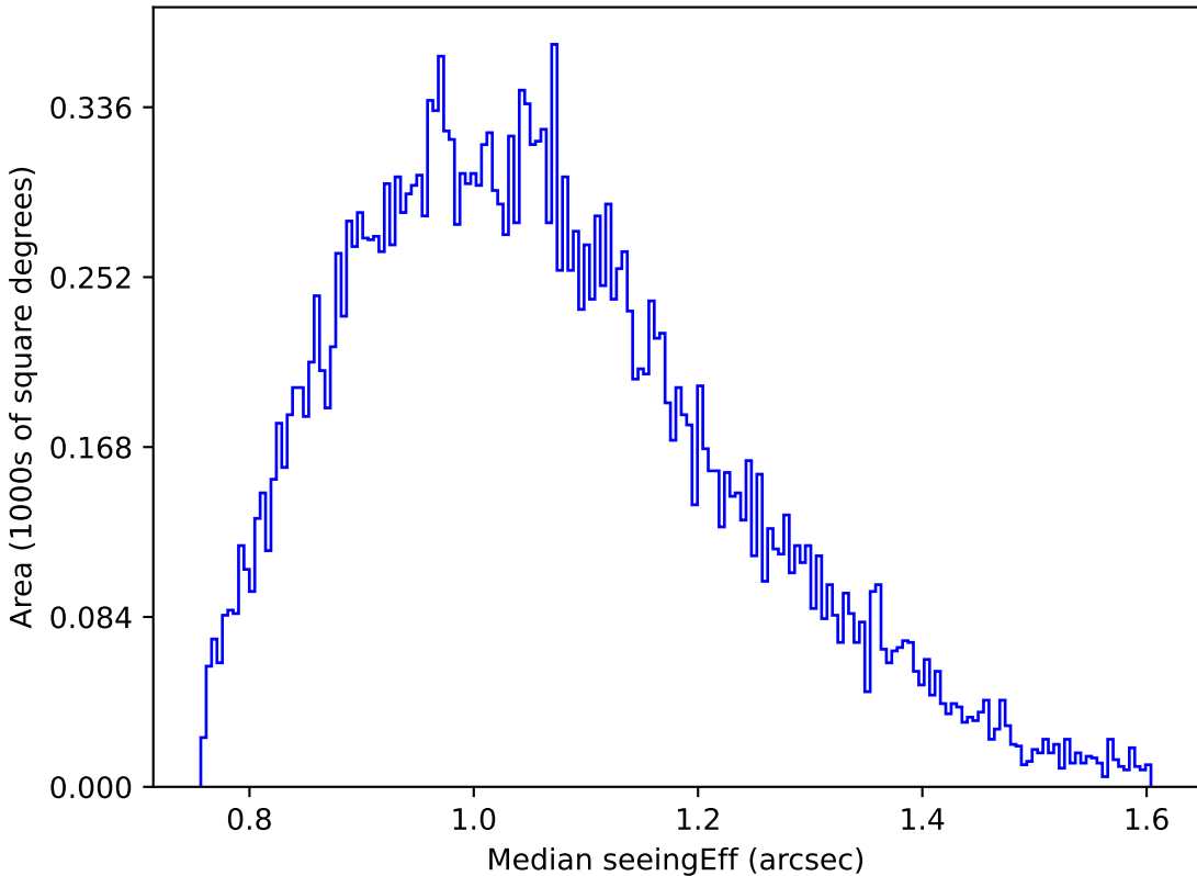
too_elab_r16_d3_ugrizy_v3.4_10yrs Yr 1 g band: Median seeingEff
