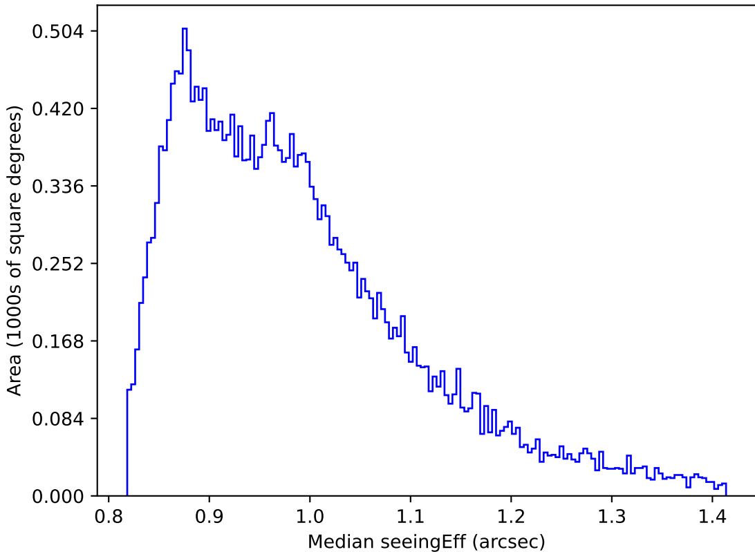
too_elab_r16_d3_ugrizy_v3.4_10yrs Yr 1 all bands: Median seeingEff
