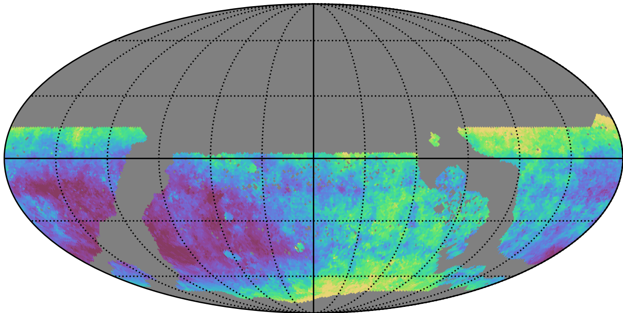
too_elab_r16_d3_ugrizy_v3.4_10yrs WFD z band: Median seeingEff
