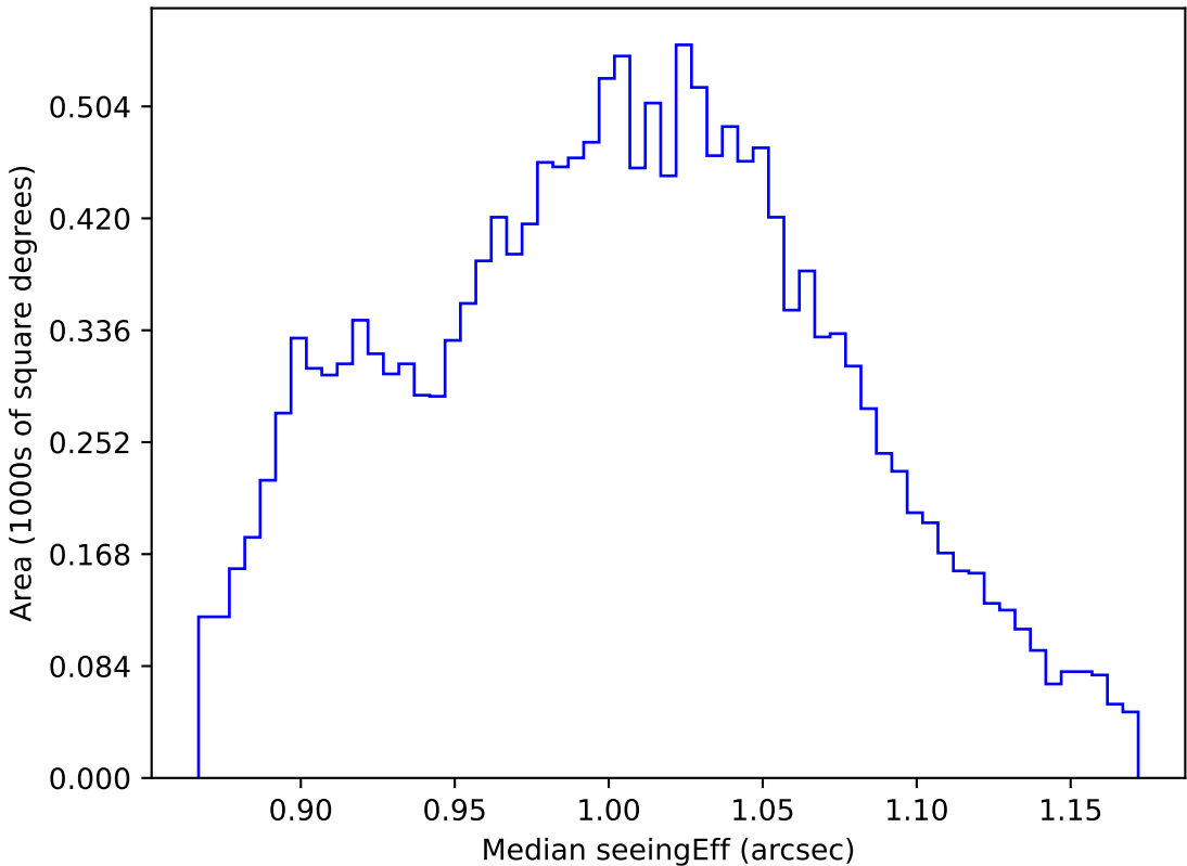
too_elab_r16_d3_ugrizy_v3.4_10yrs WFD z band: Median seeingEff
