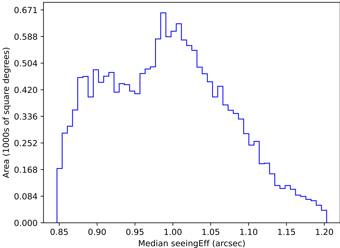
too_elab_r16_d3_ugrizy_v3.4_10yrs WFD i band: Median seeingEff
