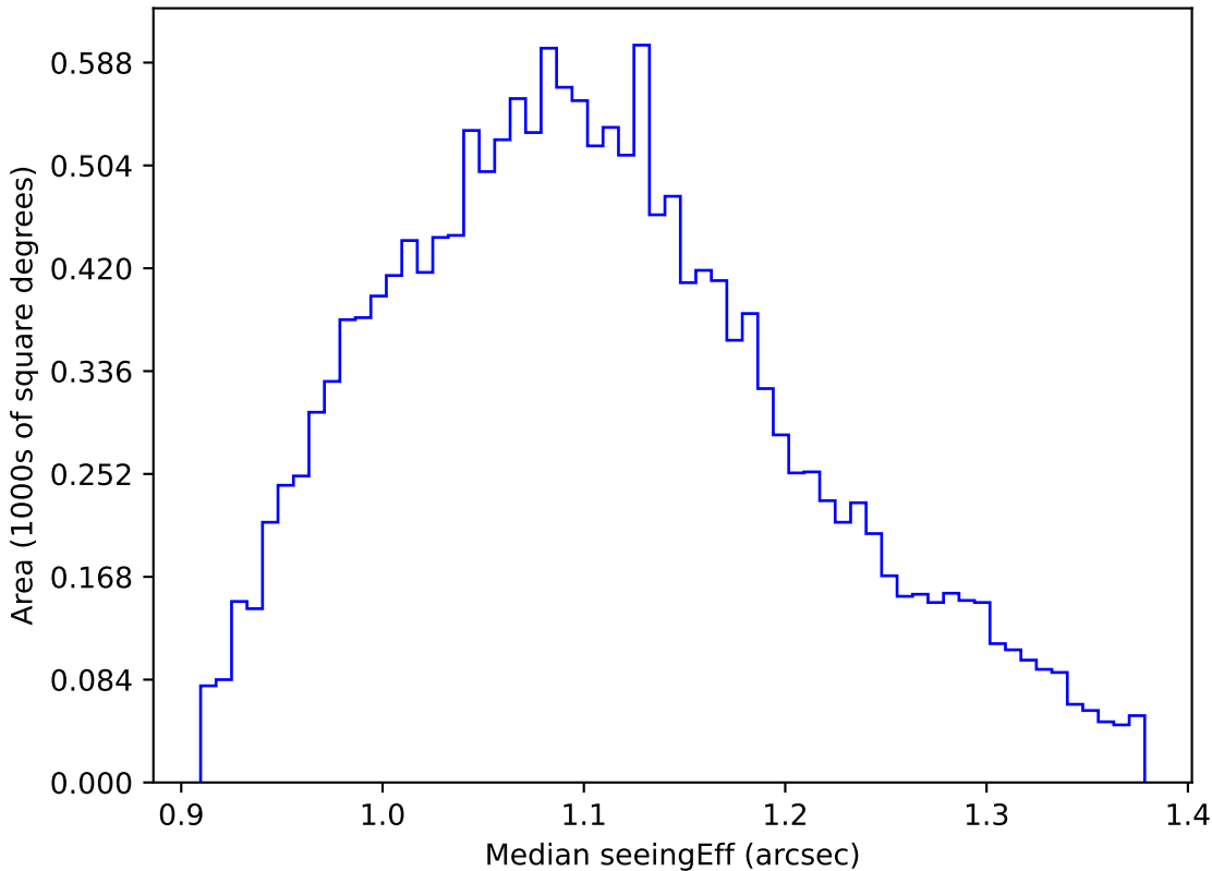
too_elab_r16_d3_ugrizy_v3.4_10yrs WFD g band: Median seeingEff
