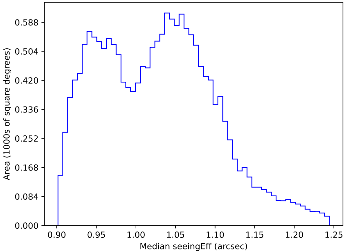
too_elab_r16_d3_ugrizy_v3.4_10yrs WFD all bands: Median seeingEff
