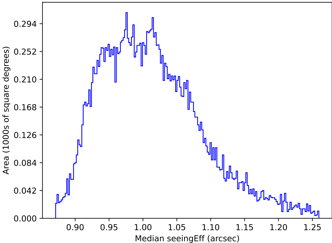
too_elab_r16_d3_ugrizy_v3.4_10yrs All sky y band: Median seeingEff
