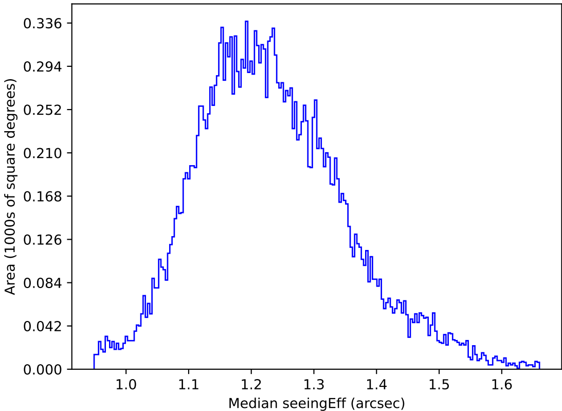
too_elab_r16_d3_ugrizy_v3.4_10yrs All sky u band: Median seeingEff
