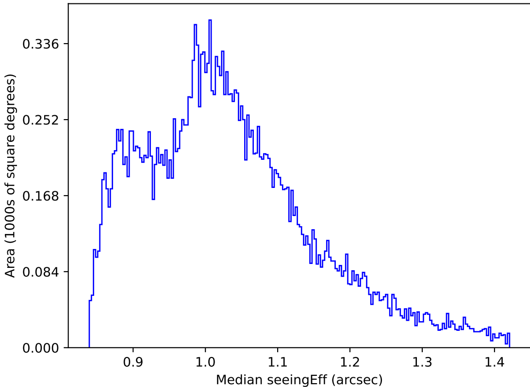
too_elab_r16_d3_ugrizy_v3.4_10yrs All sky i band: Median seeingEff
