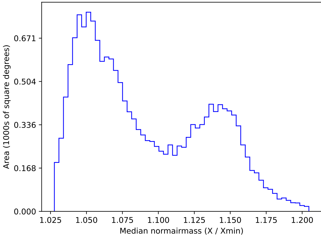
too_elab_r16_d3_ugrizy_v3.4_10yrs WFD y band: Median normairmass
