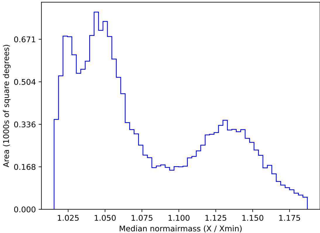
too_elab_r16_d3_ugrizy_v3.4_10yrs WFD r band: Median normairmass
