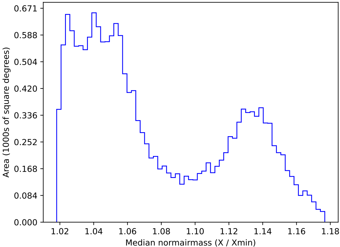
too_elab_r16_d3_ugrizy_v3.4_10yrs WFD i band: Median normairmass
