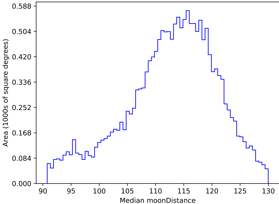
too_elab_r16_d3_ugrizy_v3.4_10yrs WFD r band: Median moonDistance
