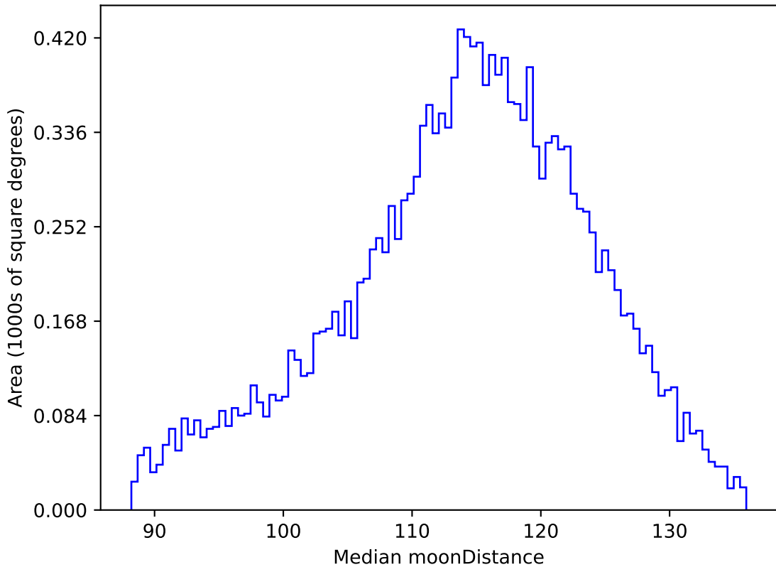
too_elab_r16_d3_ugrizy_v3.4_10yrs WFD g band: Median moonDistance
