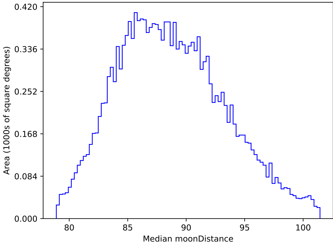
too_elab_r16_d3_ugrizy_v3.4_10yrs WFD all bands: Median moonDistance
