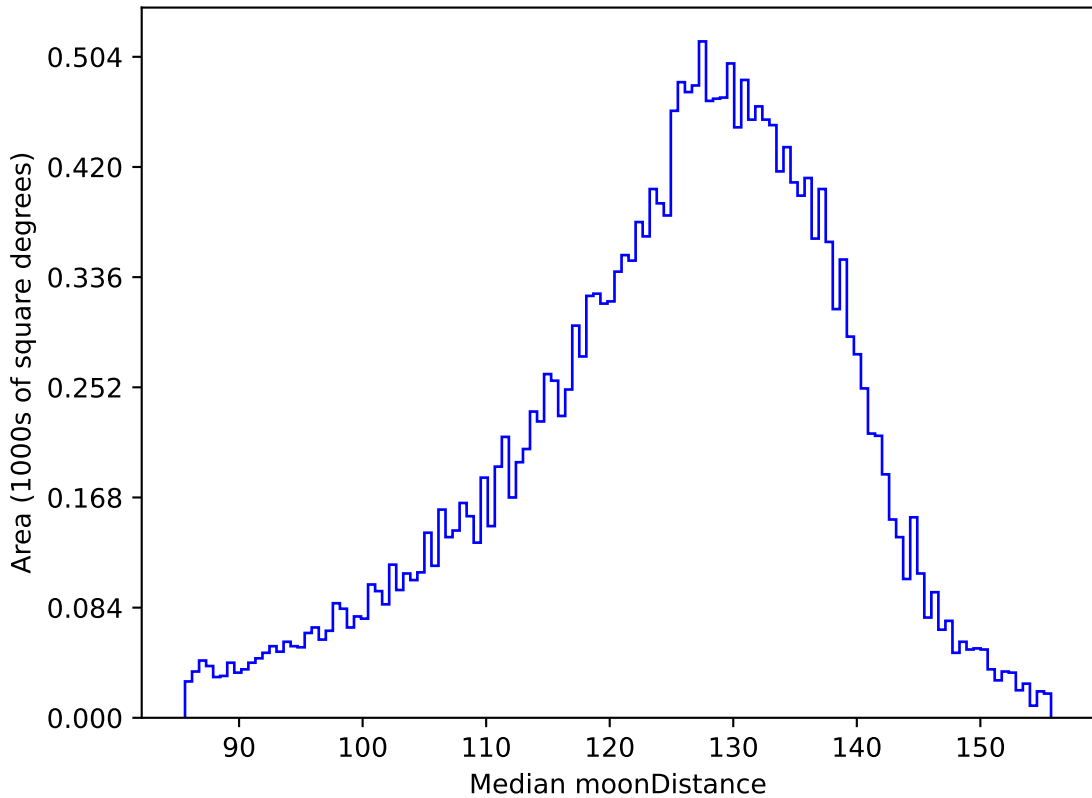
too_elab_r16_d3_ugrizy_v3.4_10yrs All sky u band: Median moonDistance
