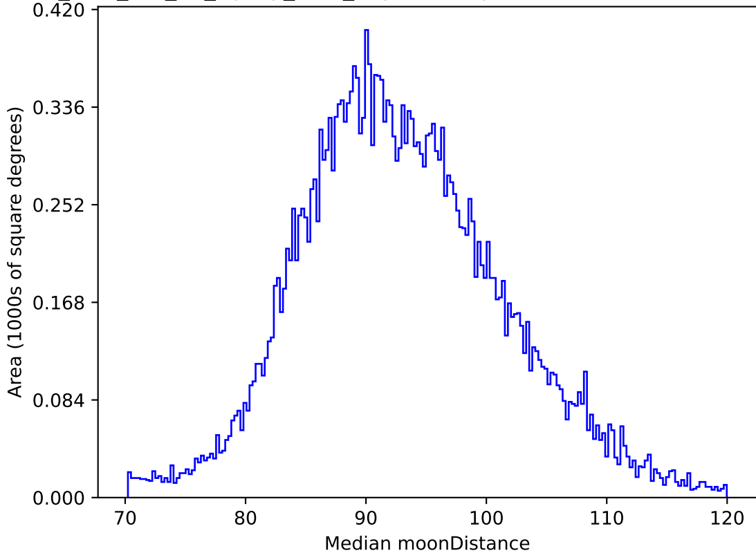
too_elab_r16_d3_ugrizy_v3.4_10yrs All sky i band: Median moonDistance
