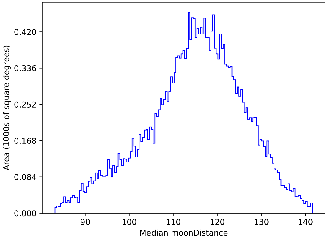
too_elab_r16_d3_ugrizy_v3.4_10yrs All sky g band: Median moonDistance
