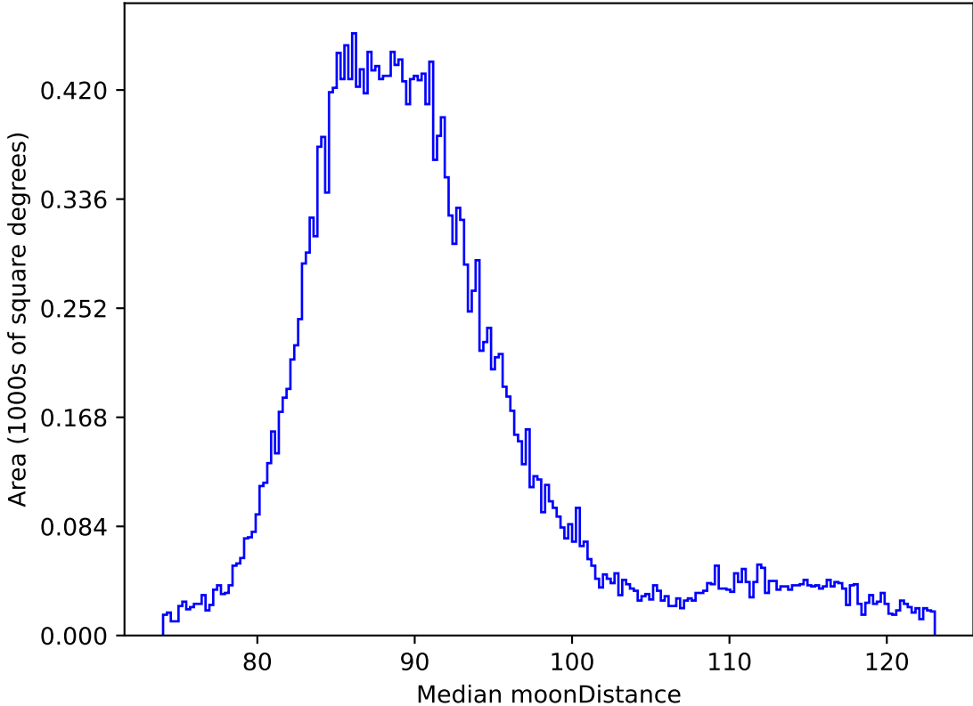
too_elab_r16_d3_ugrizy_v3.4_10yrs All sky all bands: Median moonDistance
