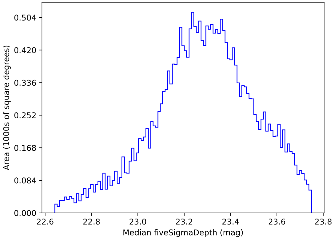
too_elab_r16_d3_ugrizy_v3.4_10yrs Yr 1 u band: Median fiveSigmaDepth
