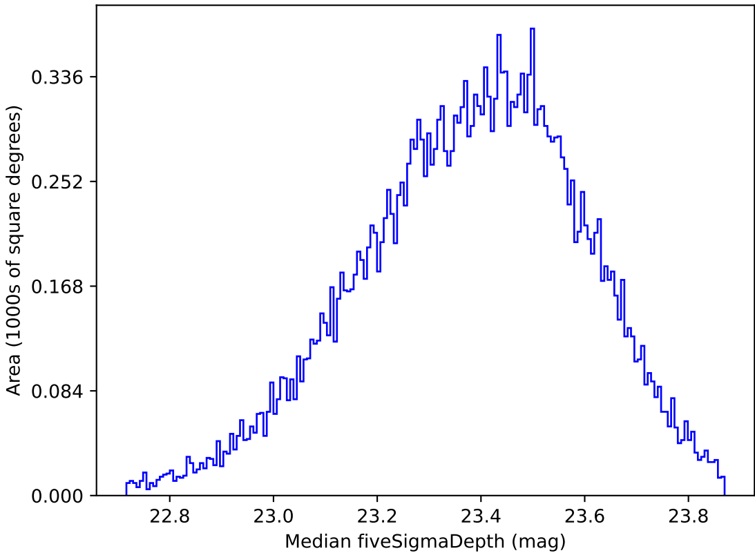
too_elab_r16_d3_ugrizy_v3.4_10yrs Yr 1 all bands: Median fiveSigmaDepth
