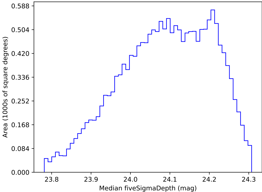
too_elab_r16_d3_ugrizy_v3.4_10yrs WFD r band: Median fiveSigmaDepth
