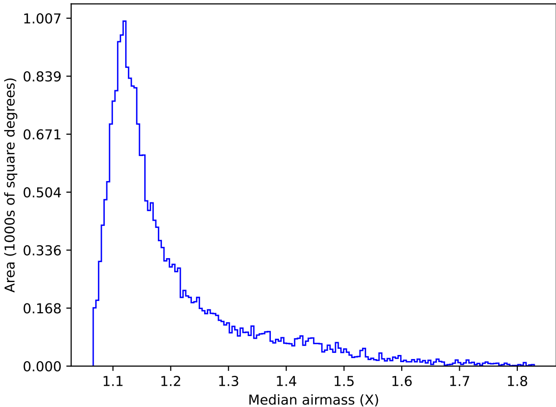
too_elab_r16_d3_ugrizy_v3.4_10yrs Yr 1 y band: Median airmass
