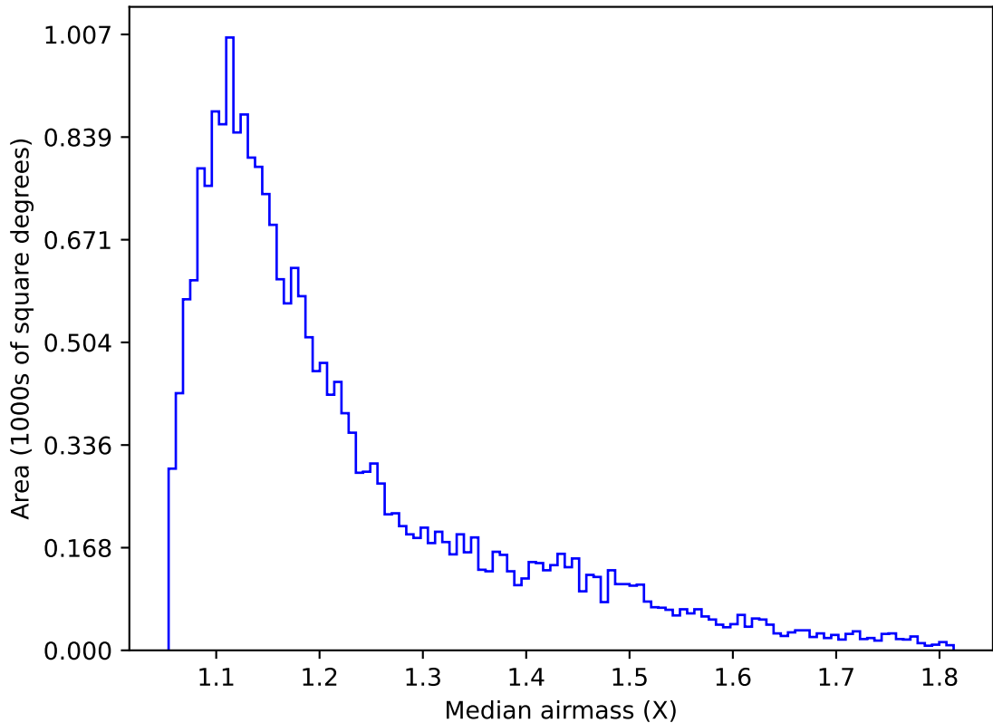
too_elab_r16_d3_ugrizy_v3.4_10yrs Yr 1 u band: Median airmass
