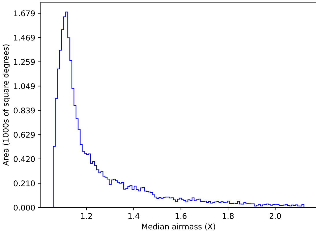
too_elab_r16_d3_ugrizy_v3.4_10yrs Yr 1 r band: Median airmass
