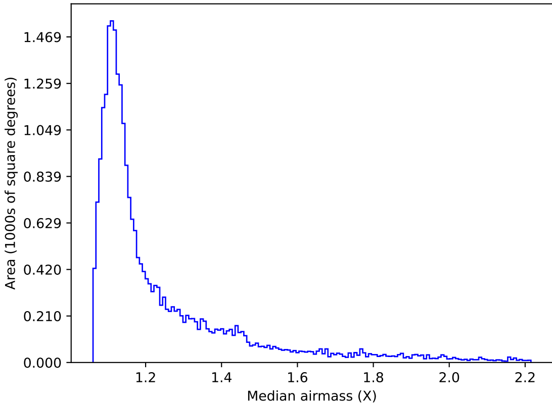
too_elab_r16_d3_ugrizy_v3.4_10yrs Yr 1 i band: Median airmass
