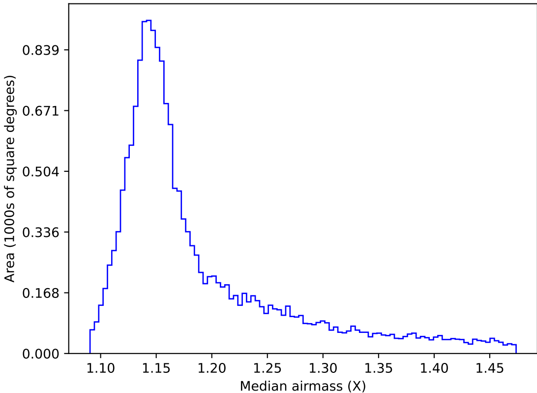
too_elab_r16_d3_ugrizy_v3.4_10yrs WFD y band: Median airmass
