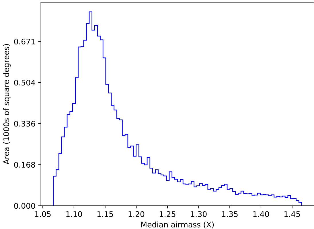
too_elab_r16_d3_ugrizy_v3.4_10yrs WFD u band: Median airmass
