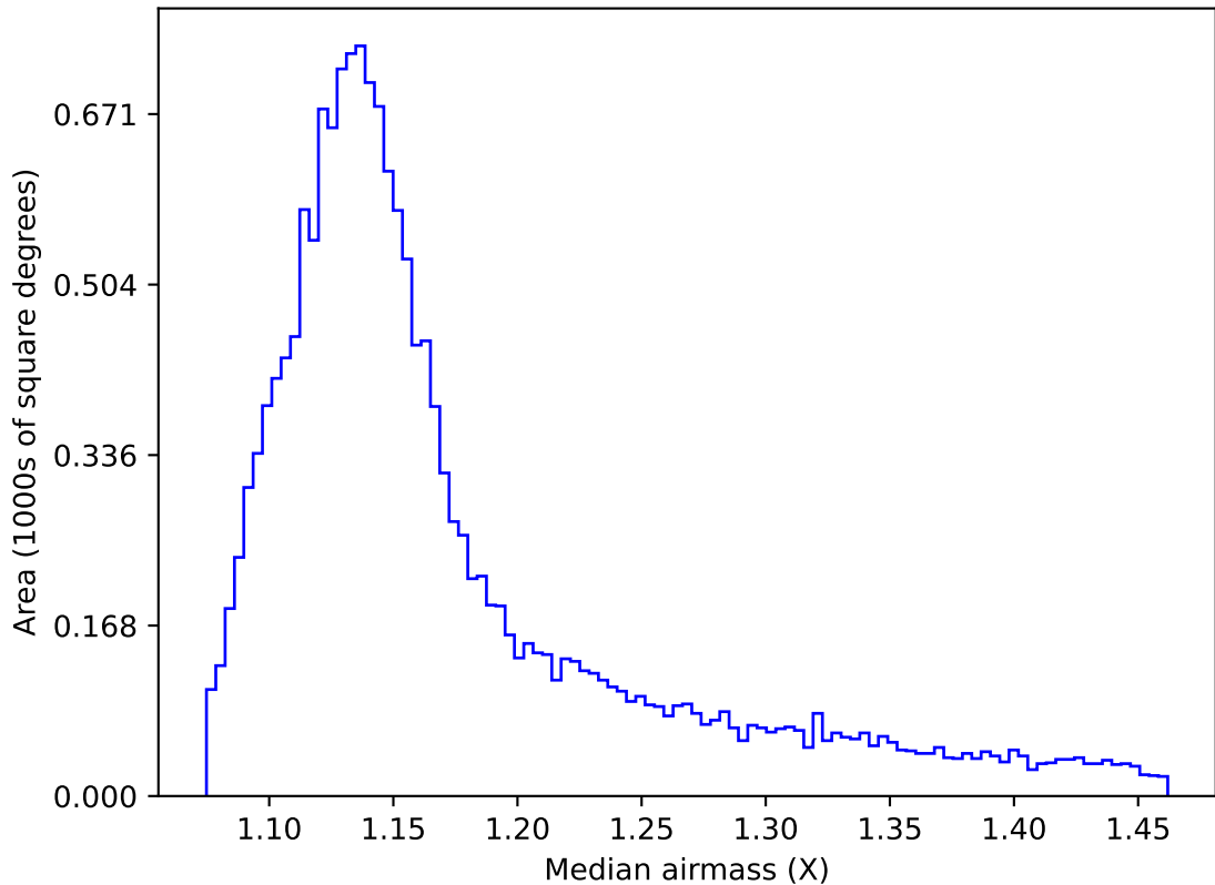
too_elab_r16_d3_ugrizy_v3.4_10yrs WFD r band: Median airmass
