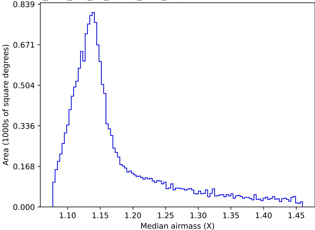
too_elab_r16_d3_ugrizy_v3.4_10yrs WFD i band: Median airmass
