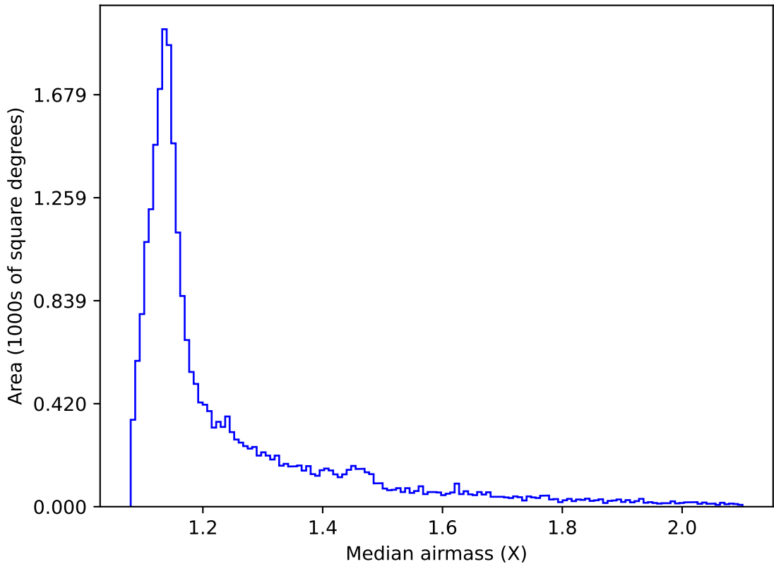
too_elab_r16_d3_ugrizy_v3.4_10yrs All sky i band: Median airmass
