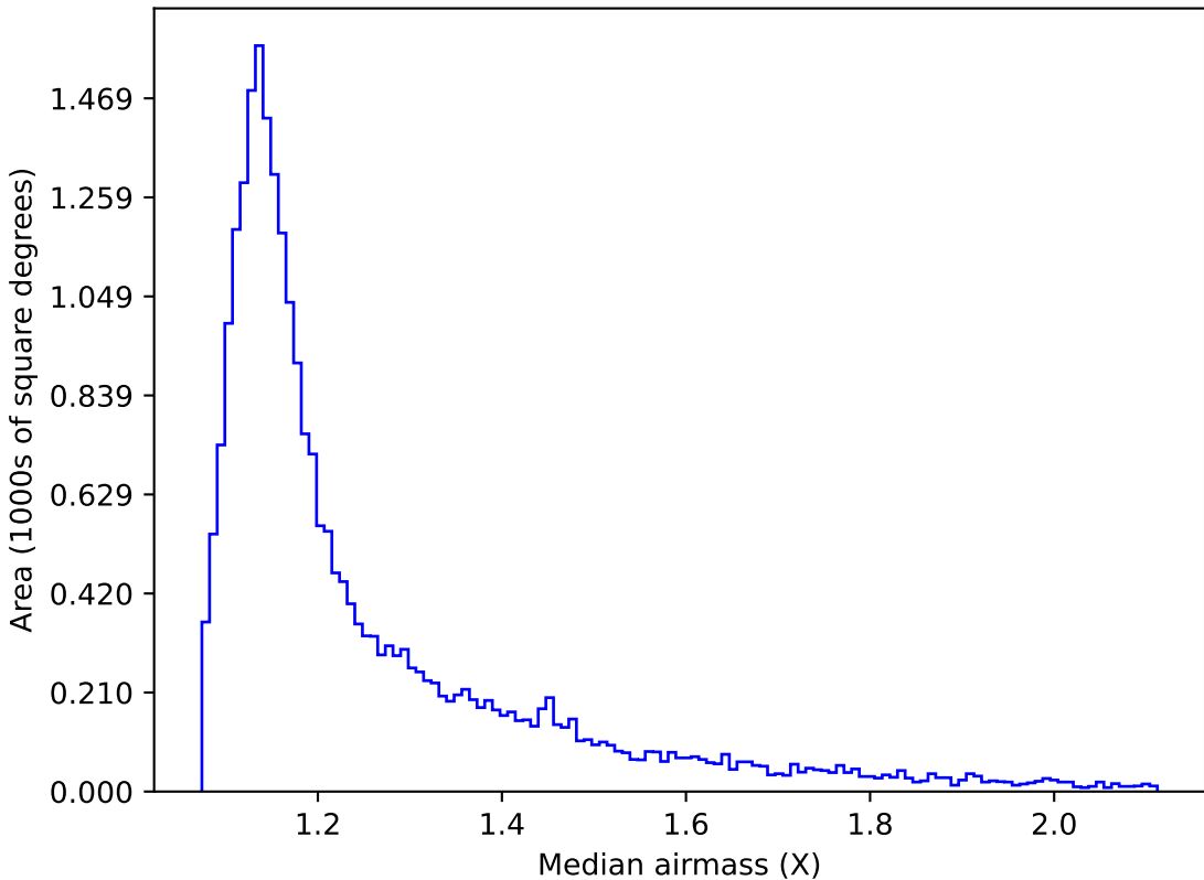
too_elab_r16_d3_ugrizy_v3.4_10yrs All sky g band: Median airmass
