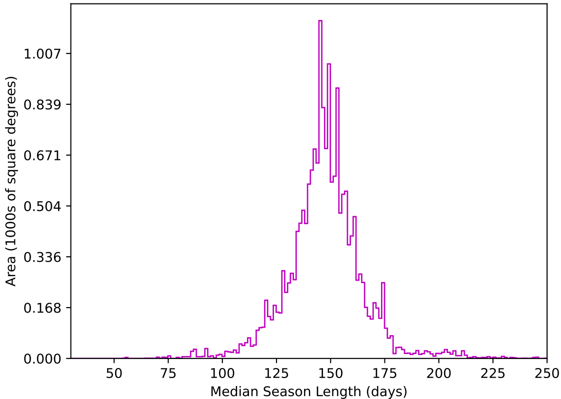
too_elab_r16_d3_ugrizy_v3.4_10yrs WFD z band: Median Season Length
