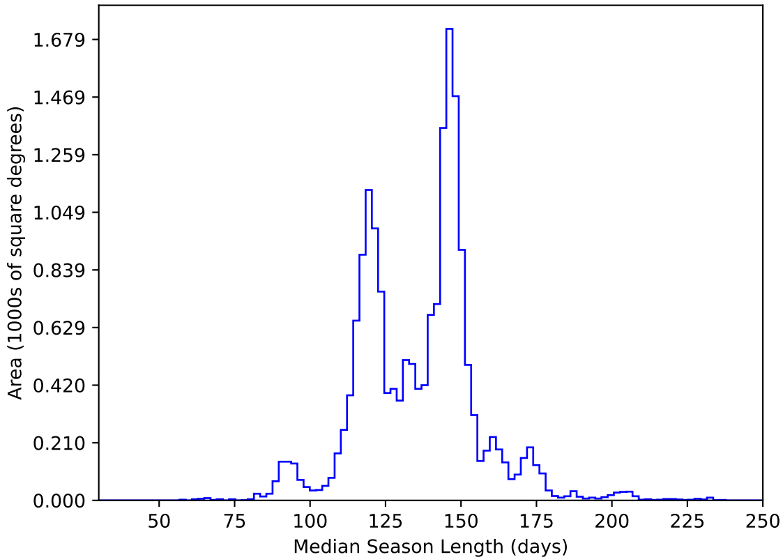
too_elab_r16_d3_ugrizy_v3.4_10yrs WFD y band: Median Season Length
