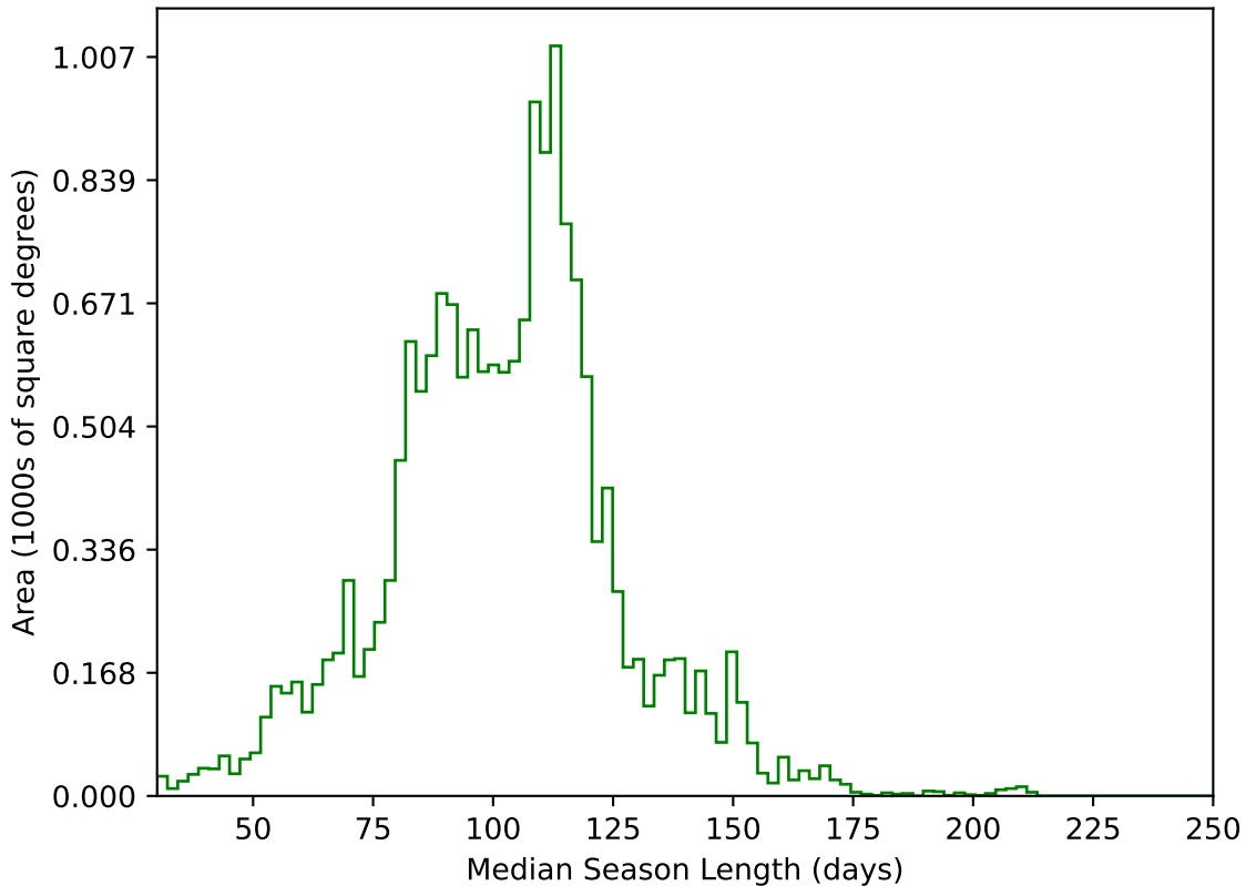
too_elab_r16_d3_ugrizy_v3.4_10yrs WFD g band: Median Season Length
