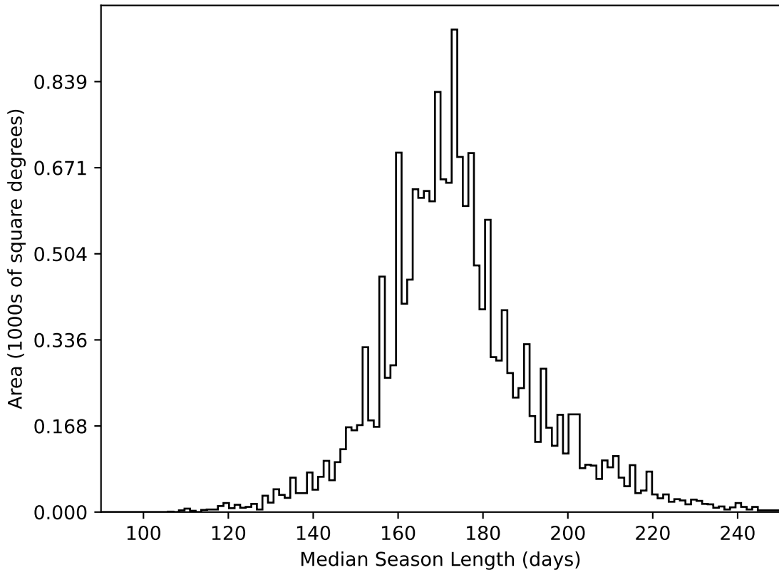
too_elab_r16_d3_ugrizy_v3.4_10yrs WFD all bands: Median Season Length
