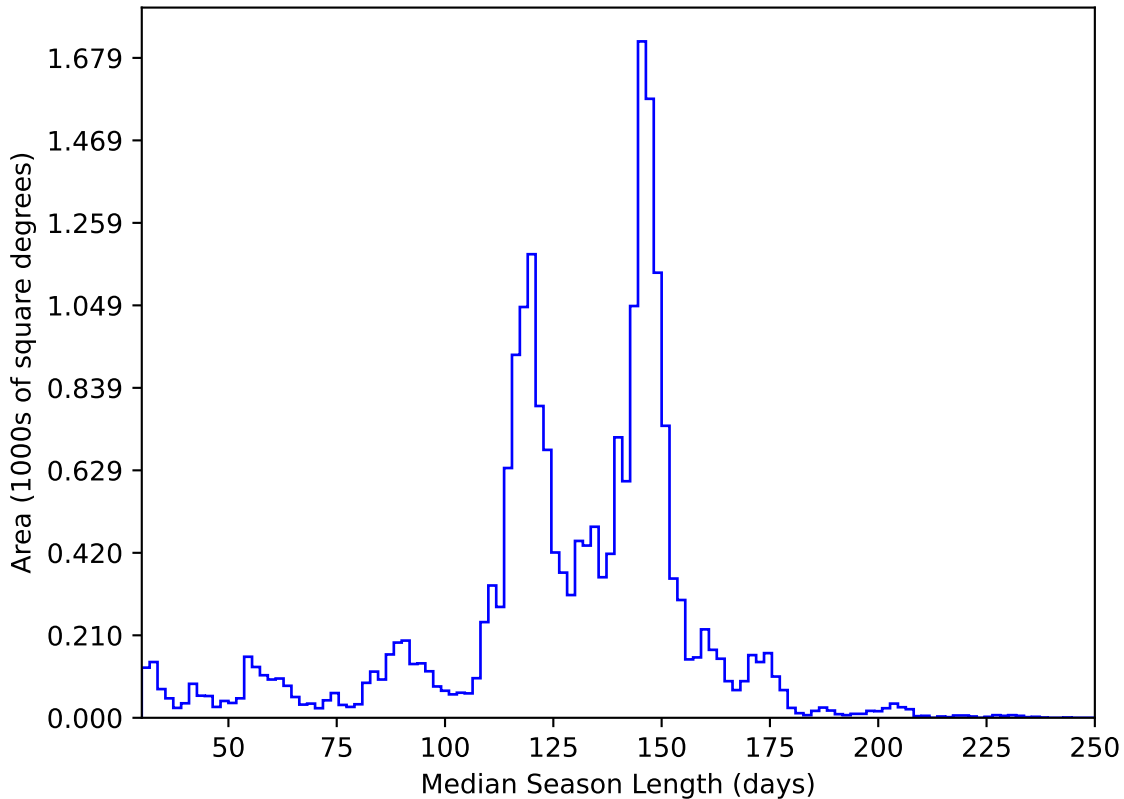
too_elab_r16_d3_ugrizy_v3.4_10yrs All sky y band: Median Season Length
