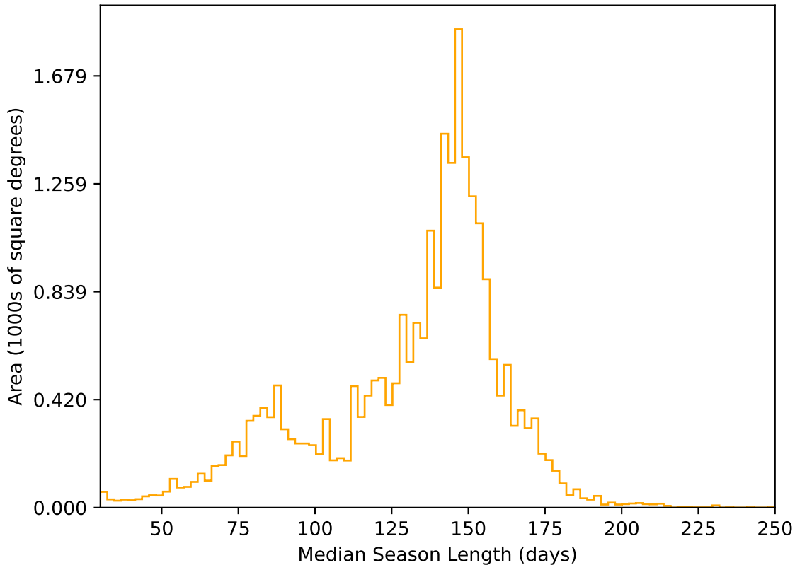
too_elab_r16_d3_ugrizy_v3.4_10yrs All sky r band: Median Season Length
