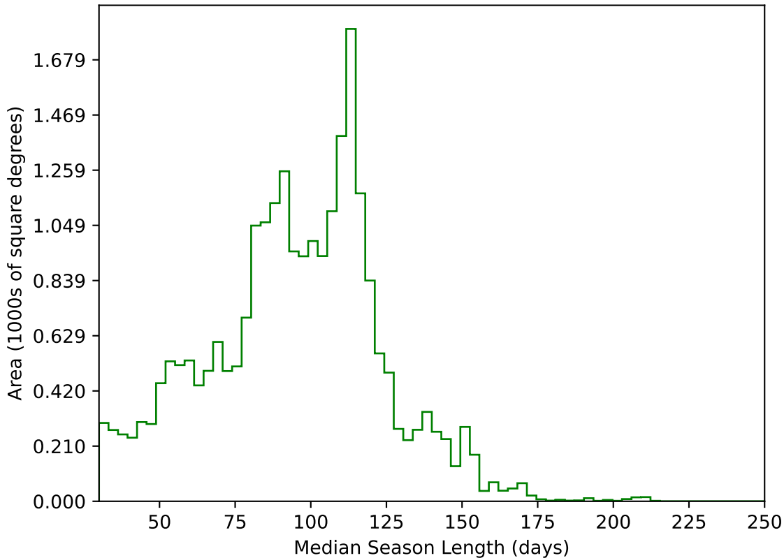
too_elab_r16_d3_ugrizy_v3.4_10yrs All sky g band: Median Season Length
