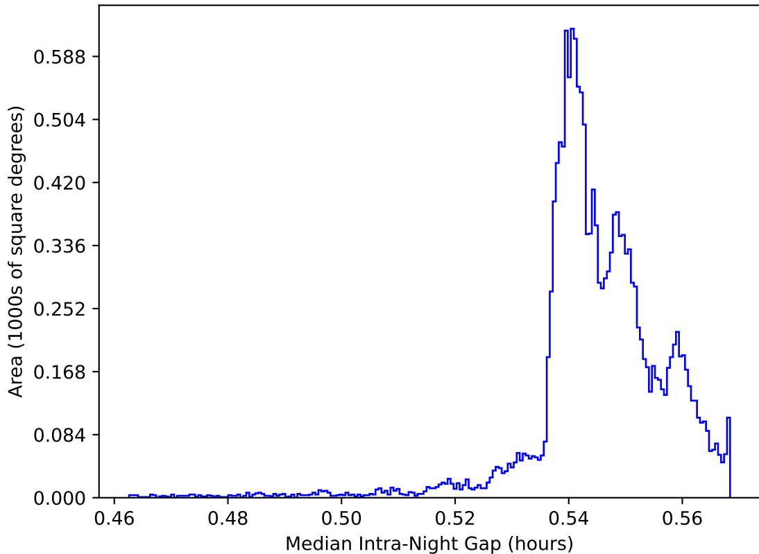
too_elab_r16_d3_ugrizy_v3.4_10yrs WFD: Median Intra-Night Gap
