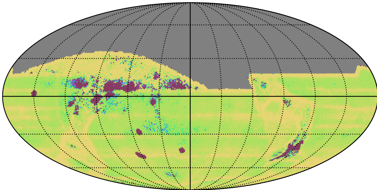
too_elab_r16_d3_ugrizy_v3.4_10yrs All sky: Median Intra-Night Gap
