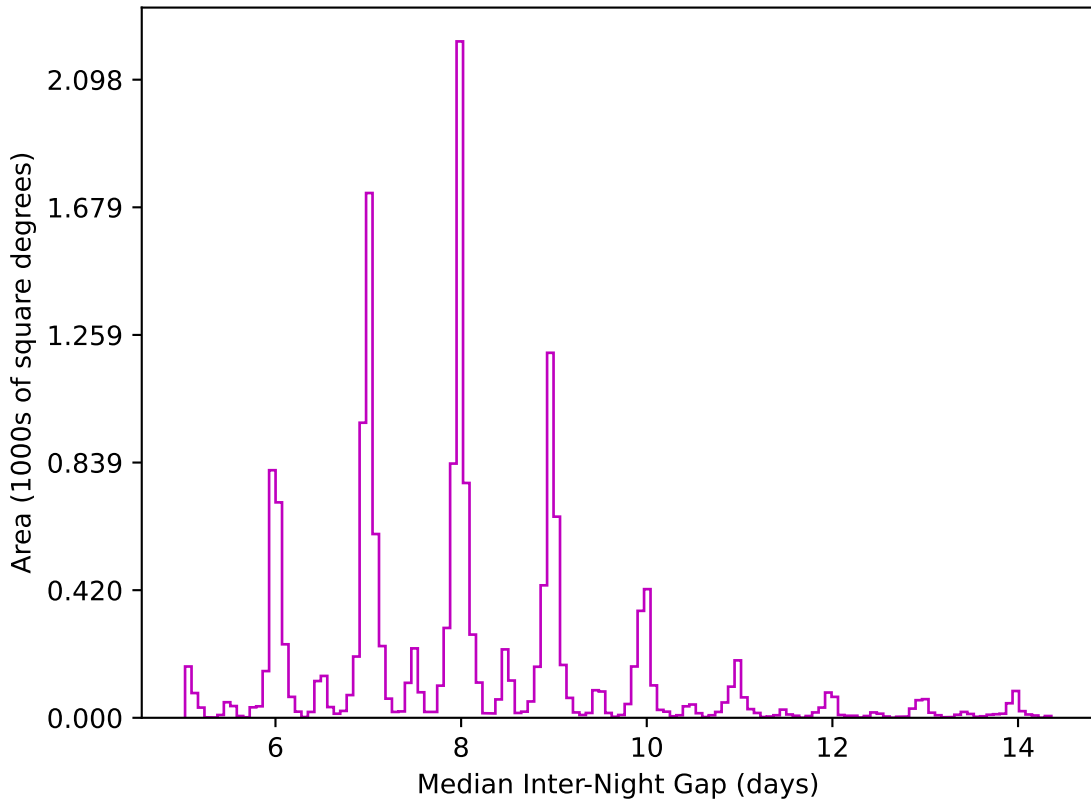
too_elab_r16_d3_ugrizy_v3.4_10yrs WFD z band: Median Inter-Night Gap
