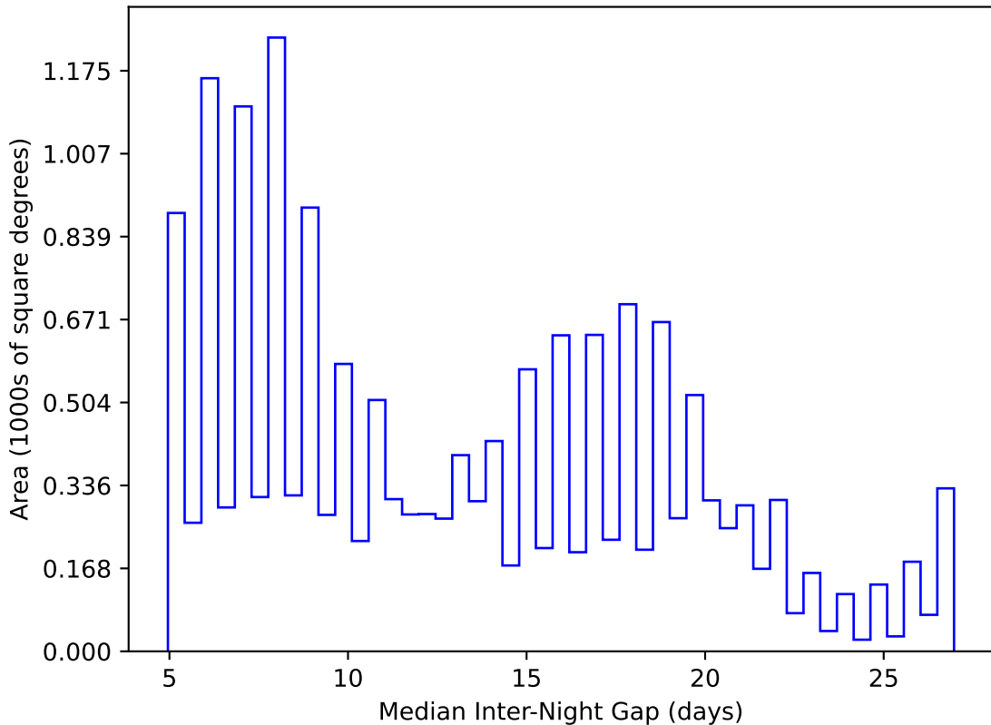
too_elab_r16_d3_ugrizy_v3.4_10yrs WFD y band: Median Inter-Night Gap
