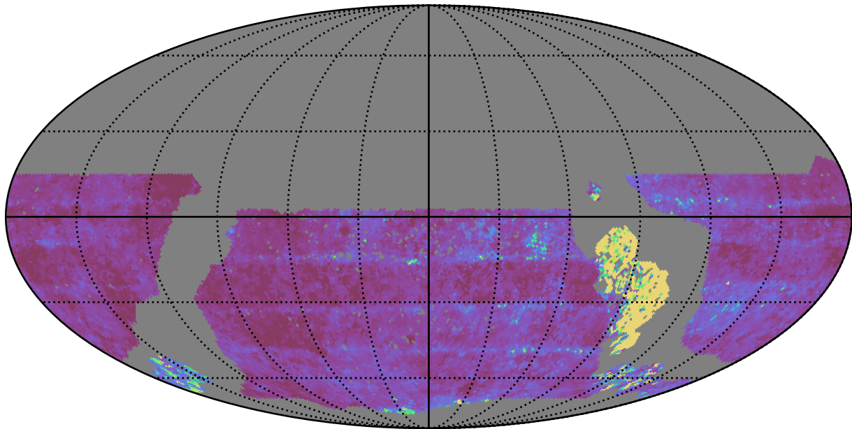
too_elab_r16_d3_ugrizy_v3.4_10yrs WFD u band: Median Inter-Night Gap
